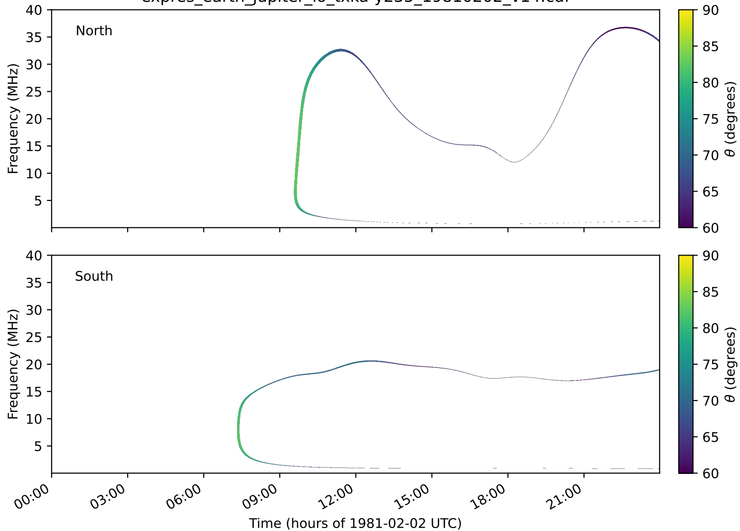
expres_earth_jupiter_io_txka-y235_19810202_v14.cdf
