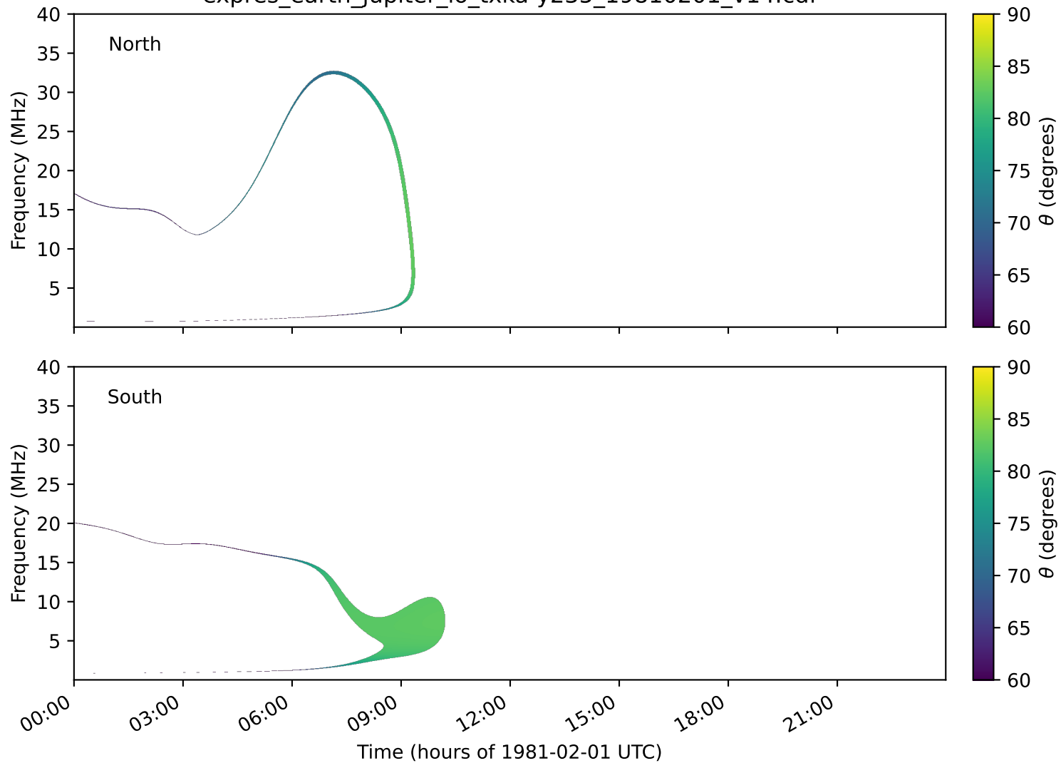
expres_earth_jupiter_io_txka-y235_19810201_v14.cdf
