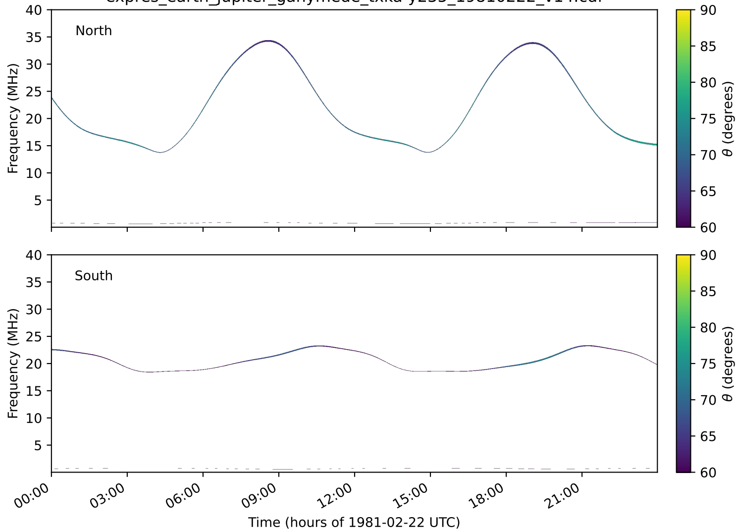
expres_earth_jupiter_ganymede_txka-y235_19810222_v14.cdf
