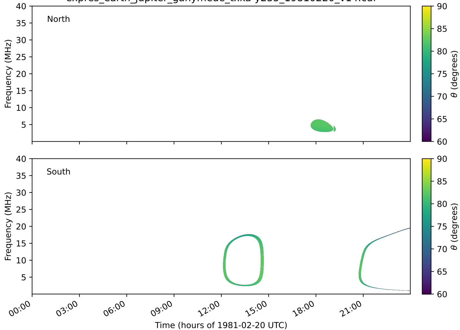
expres_earth_jupiter_ganymede_txka-y235_19810220_v14.cdf
