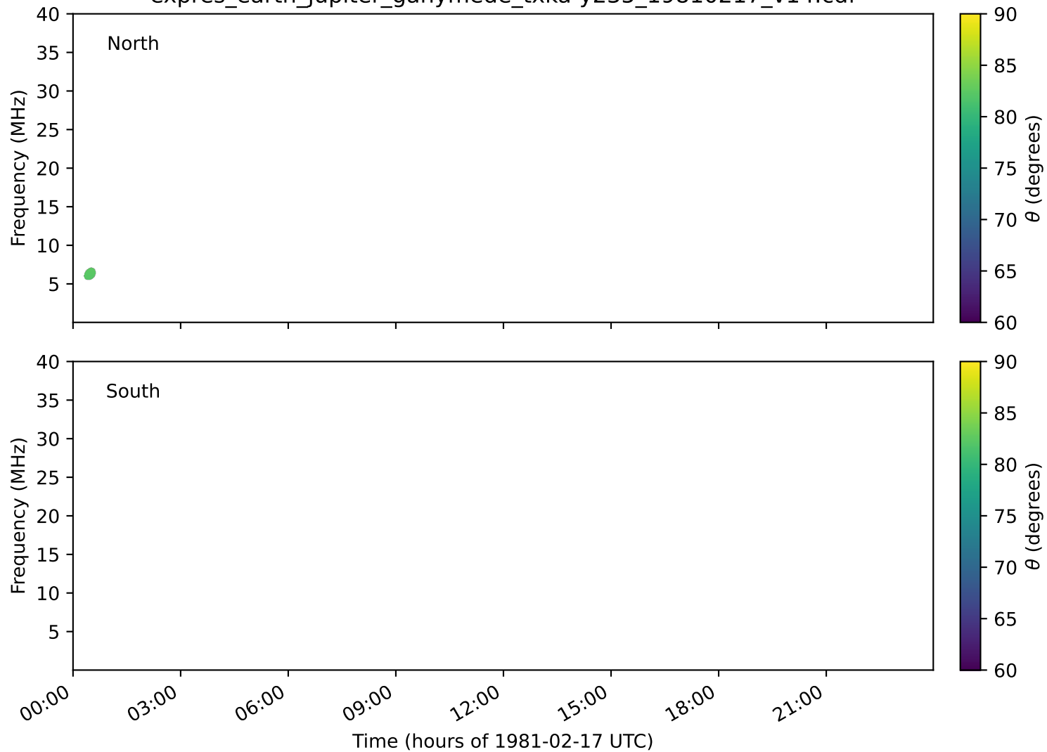
expres_earth_jupiter_ganymede_txka-y235_19810217_v14.cdf
