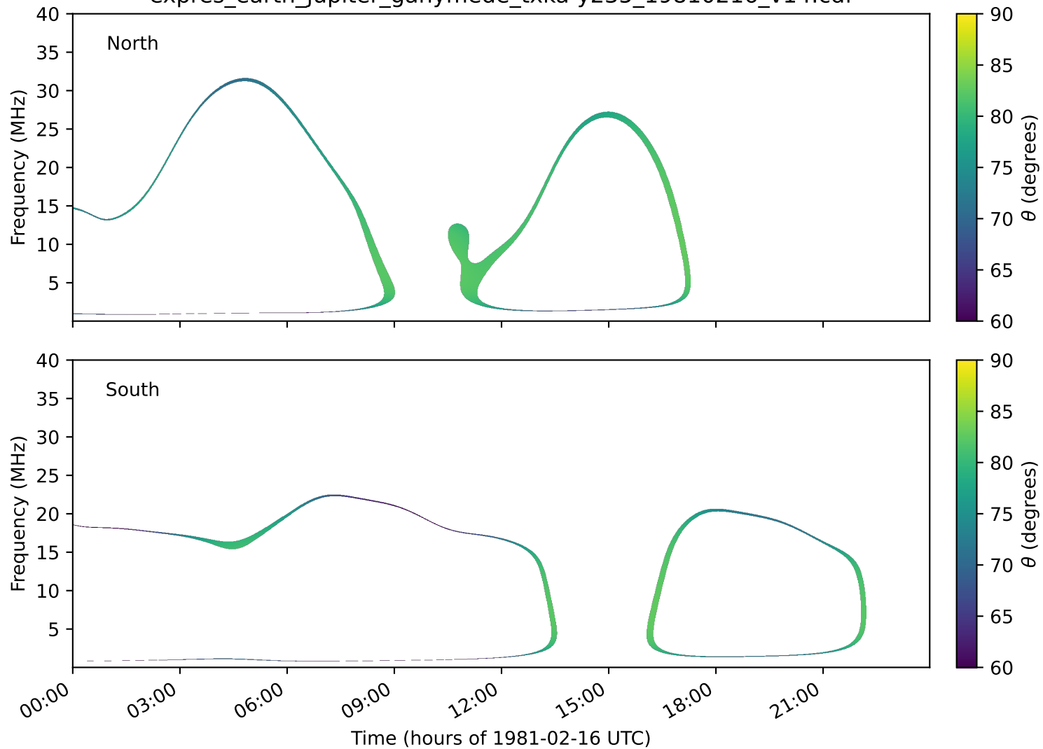
expres_earth_jupiter_ganymede_txka-y235_19810216_v14.cdf
