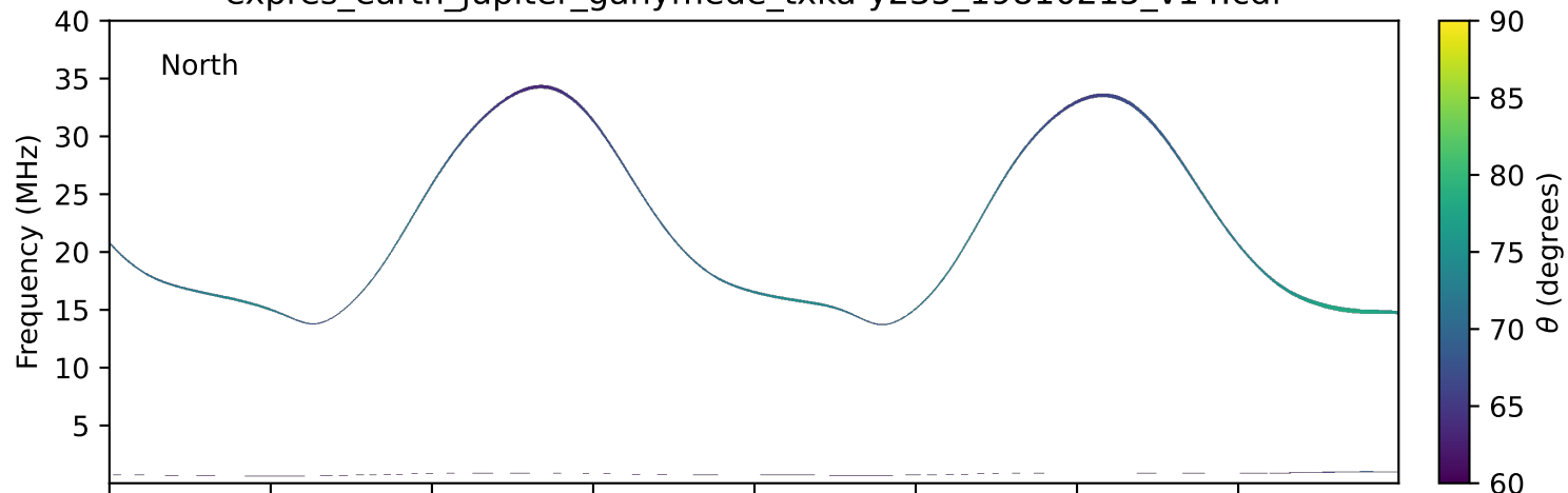
expres_earth_jupiter_ganymede_txka-y235_19810215_v14.cdf
