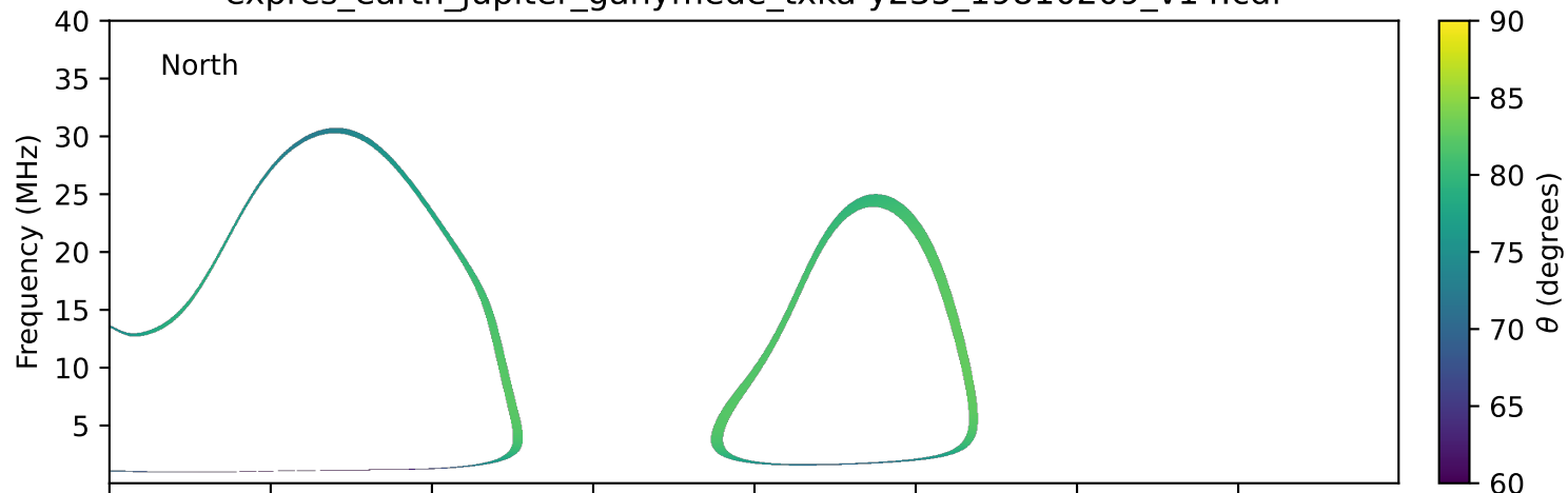
expres_earth_jupiter_ganymede_txka-y235_19810209_v14.cdf
