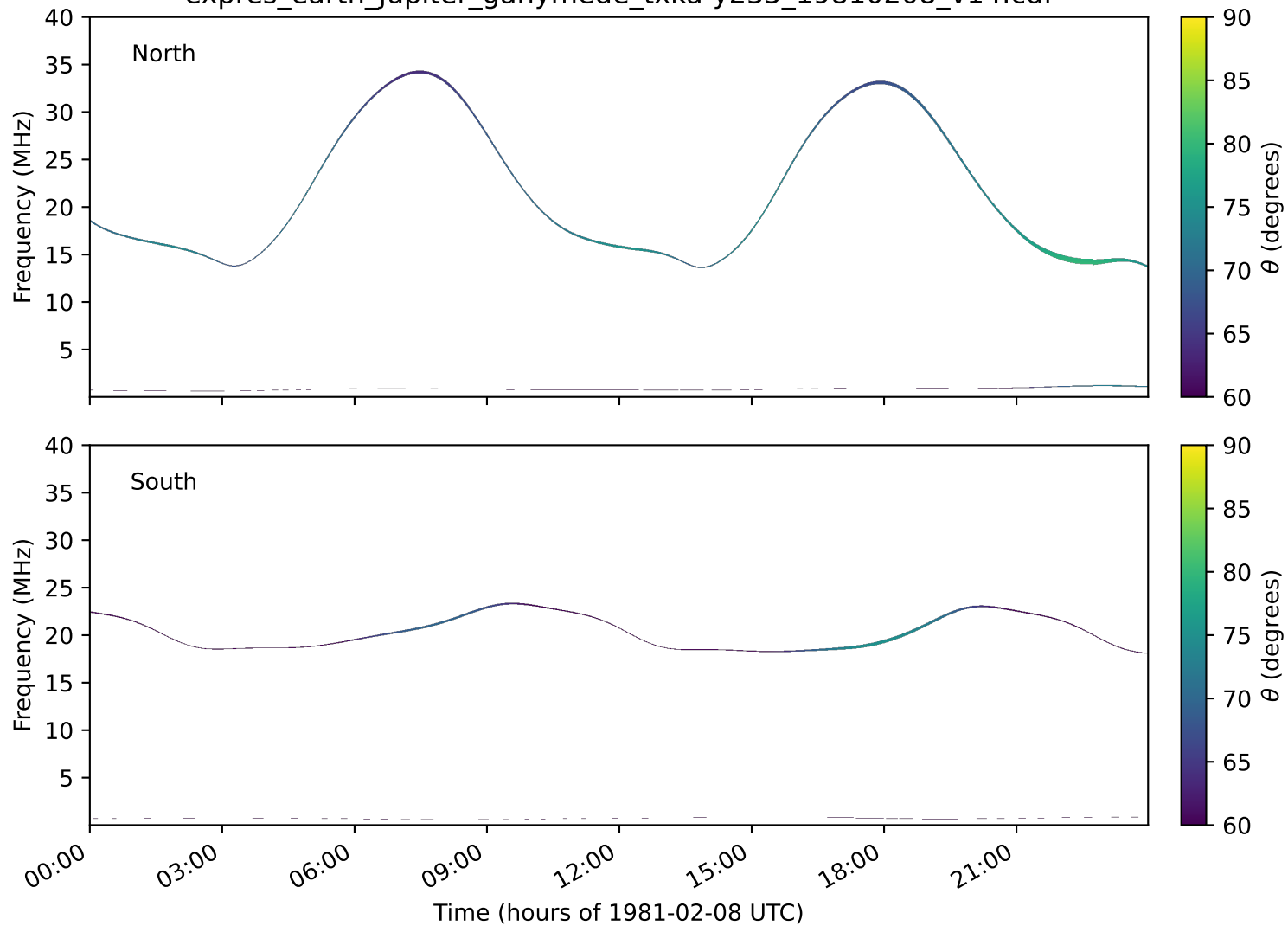
expres_earth_jupiter_ganymede_txka-y235_19810208_v14.cdf
