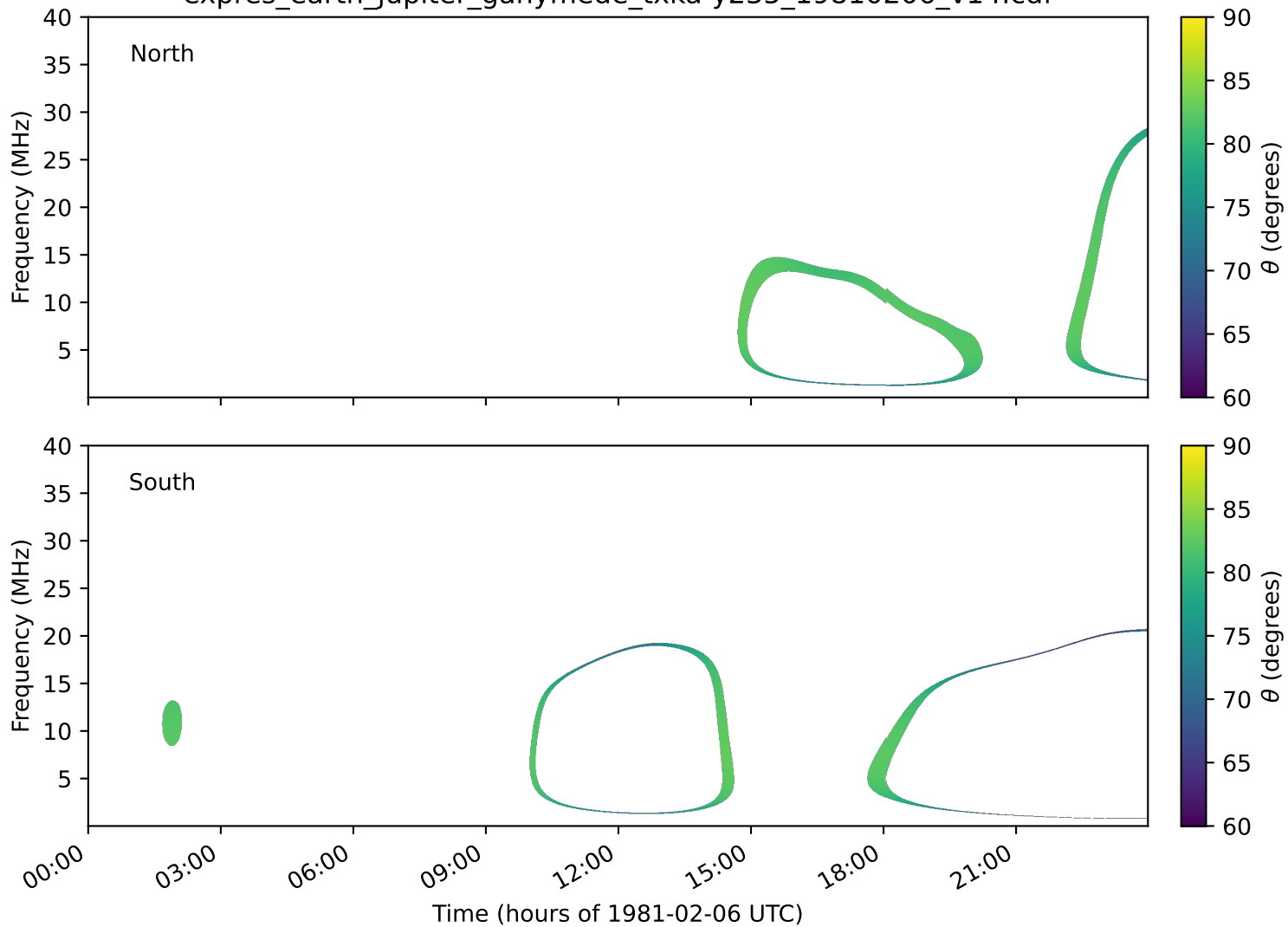
expres_earth_jupiter_ganymede_txka-y235_19810206_v14.cdf
