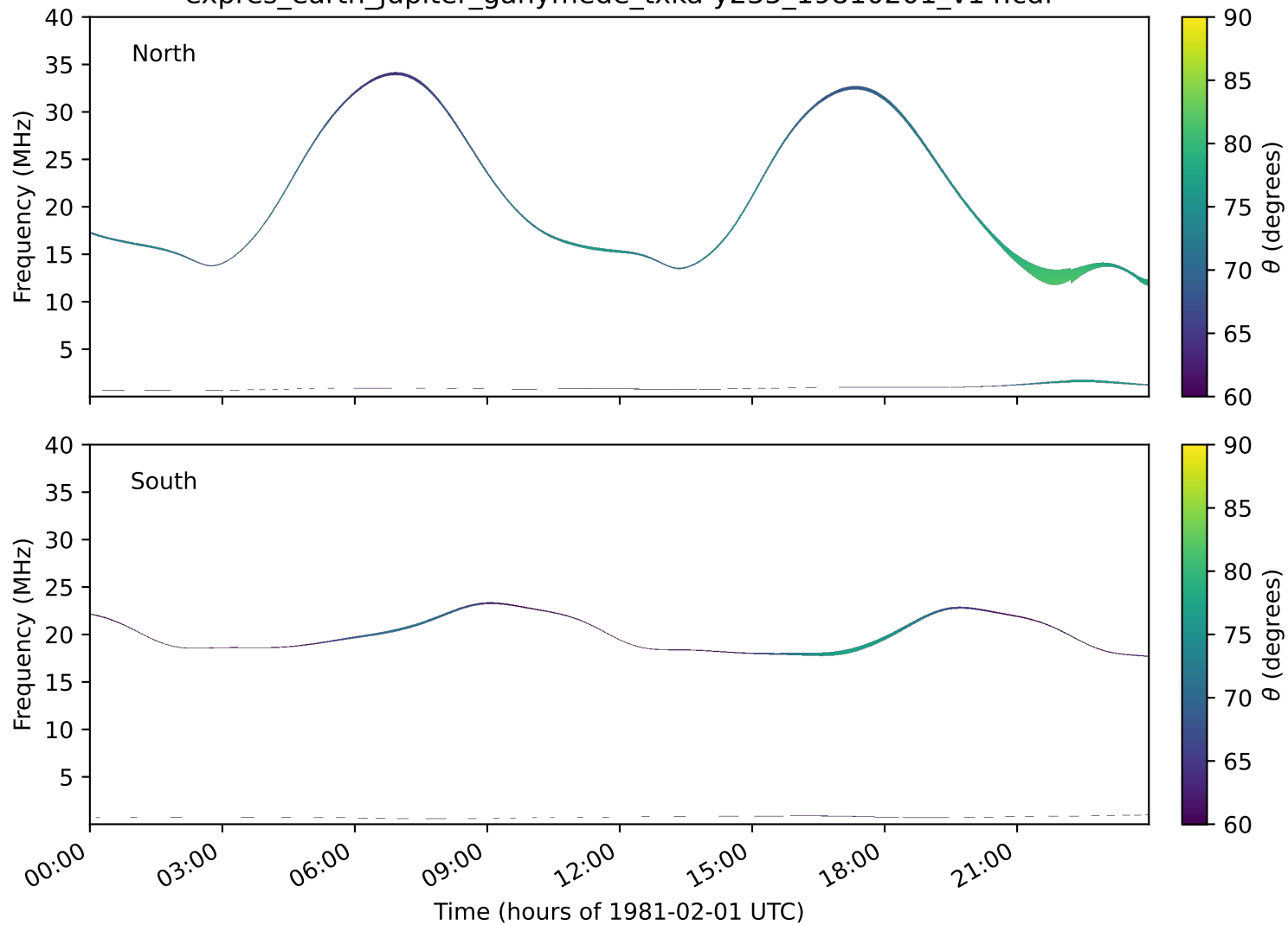
expres_earth_jupiter_ganymede_txka-y235_19810201_v14.cdf
