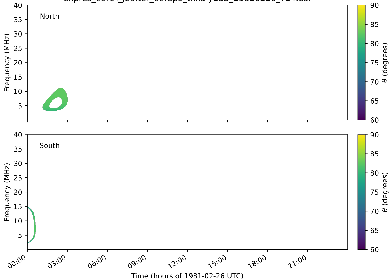
expres_earth_jupiter_europa_txka-y235_19810226_v14.cdf
