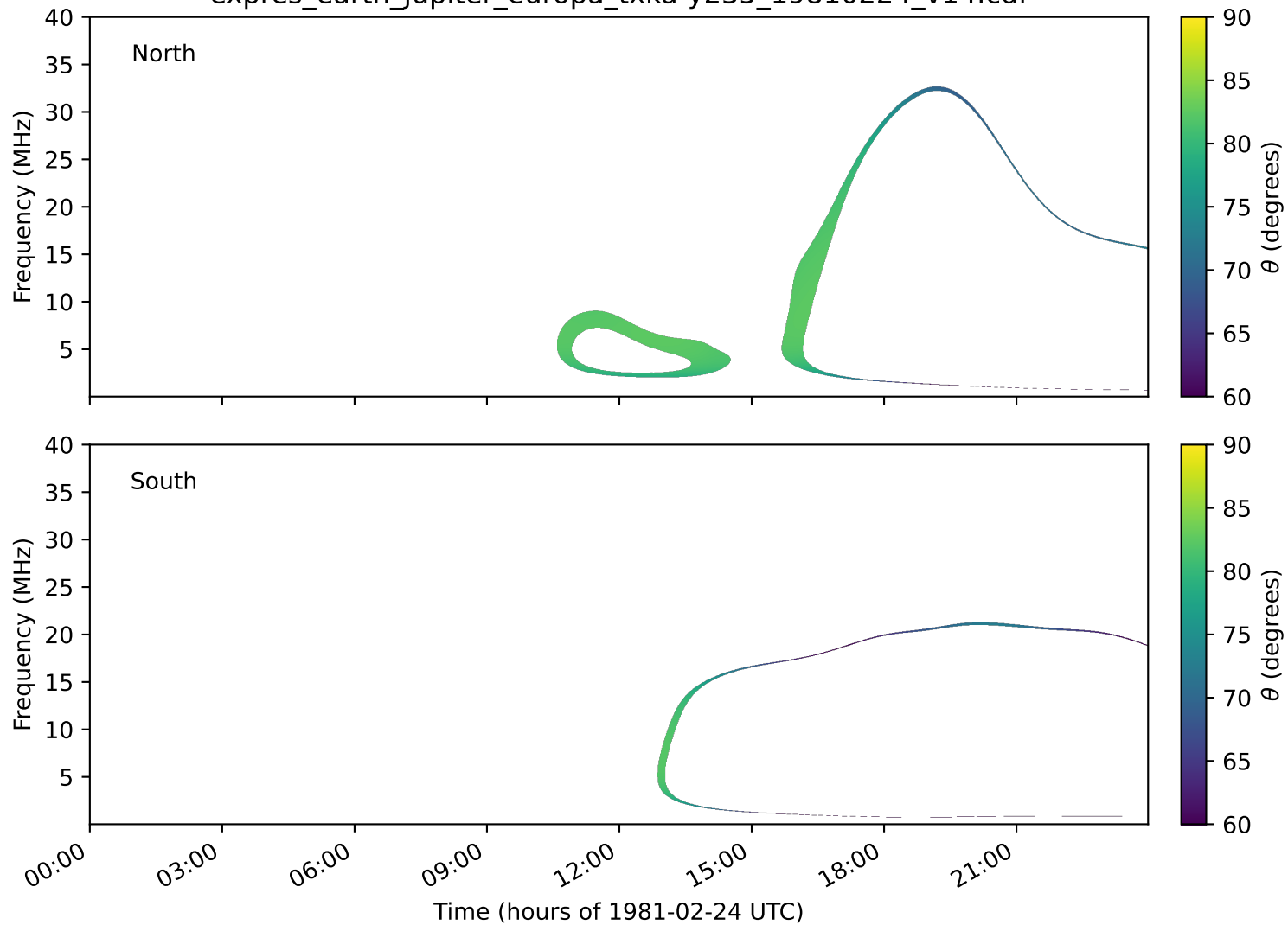
expres_earth_jupiter_europa_txka-y235_19810224_v14.cdf
