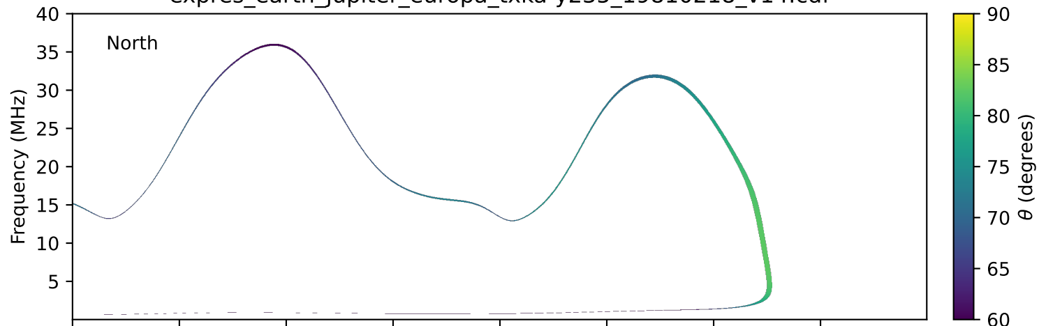
expres_earth_jupiter_europa_txka-y235_19810218_v14.cdf
