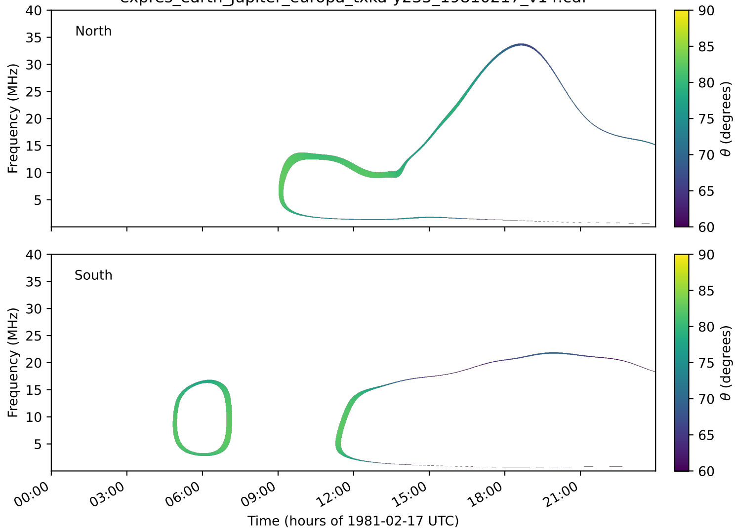
expres_earth_jupiter_europa_txka-y235_19810217_v14.cdf
