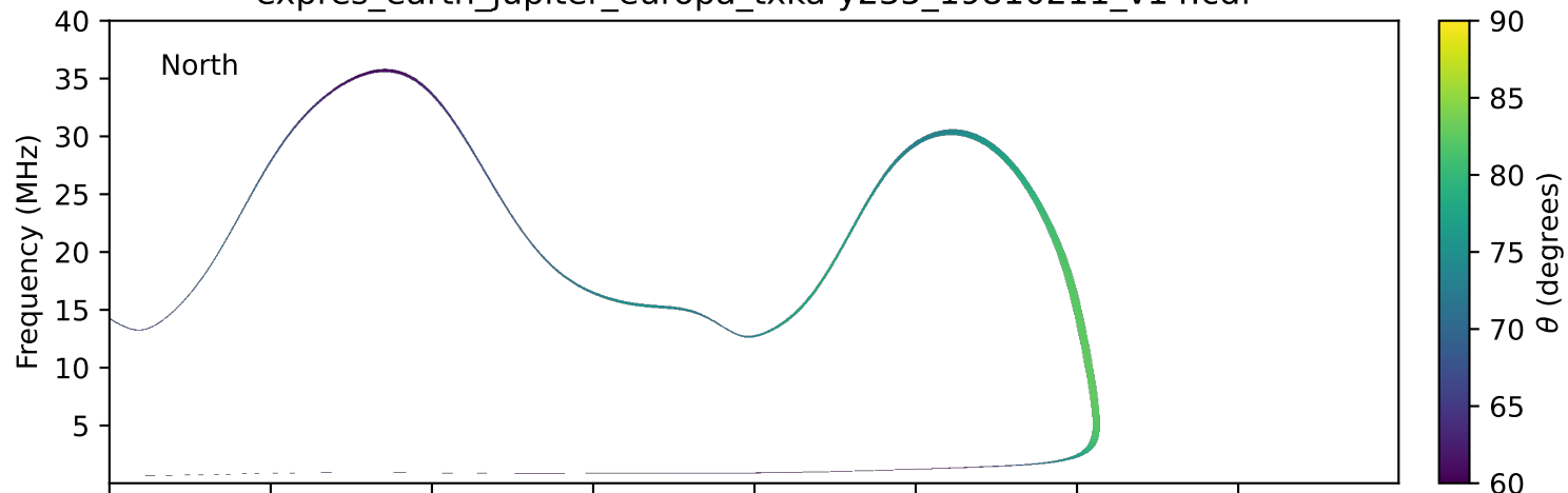
expres_earth_jupiter_europa_txka-y235_19810211_v14.cdf
