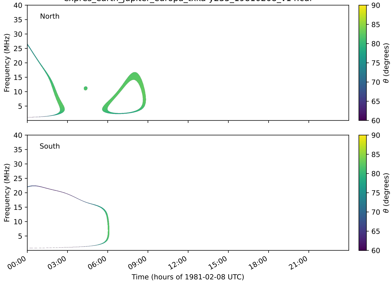
expres_earth_jupiter_europa_txka-y235_19810208_v14.cdf
