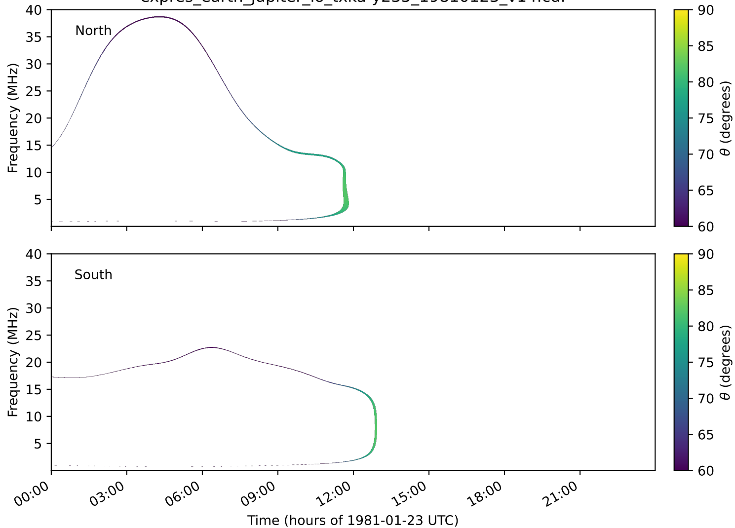
expres_earth_jupiter_io_txka-y235_19810123_v14.cdf
