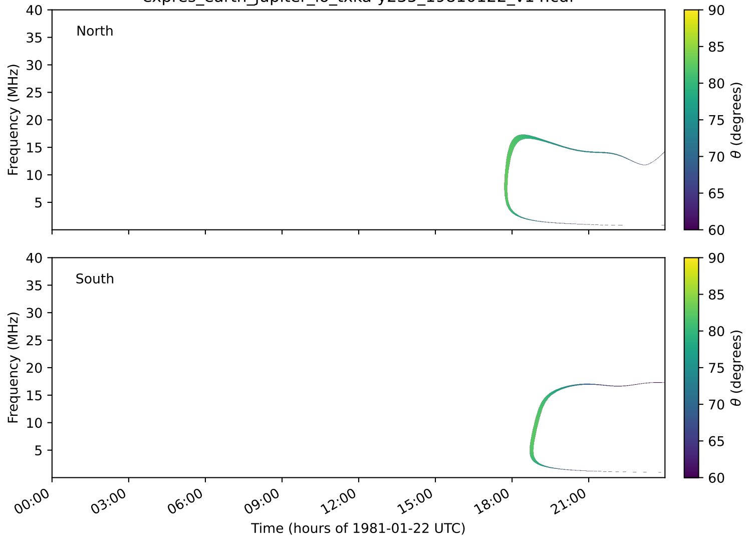
expres_earth_jupiter_io_txka-y235_19810122_v14.cdf
