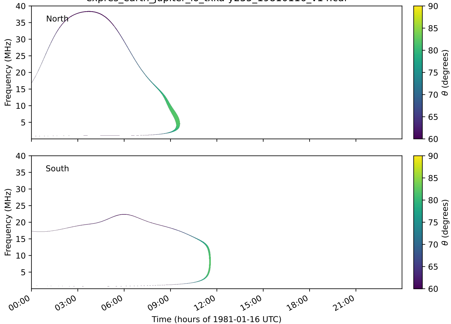
expres_earth_jupiter_io_txka-y235_19810116_v14.cdf
