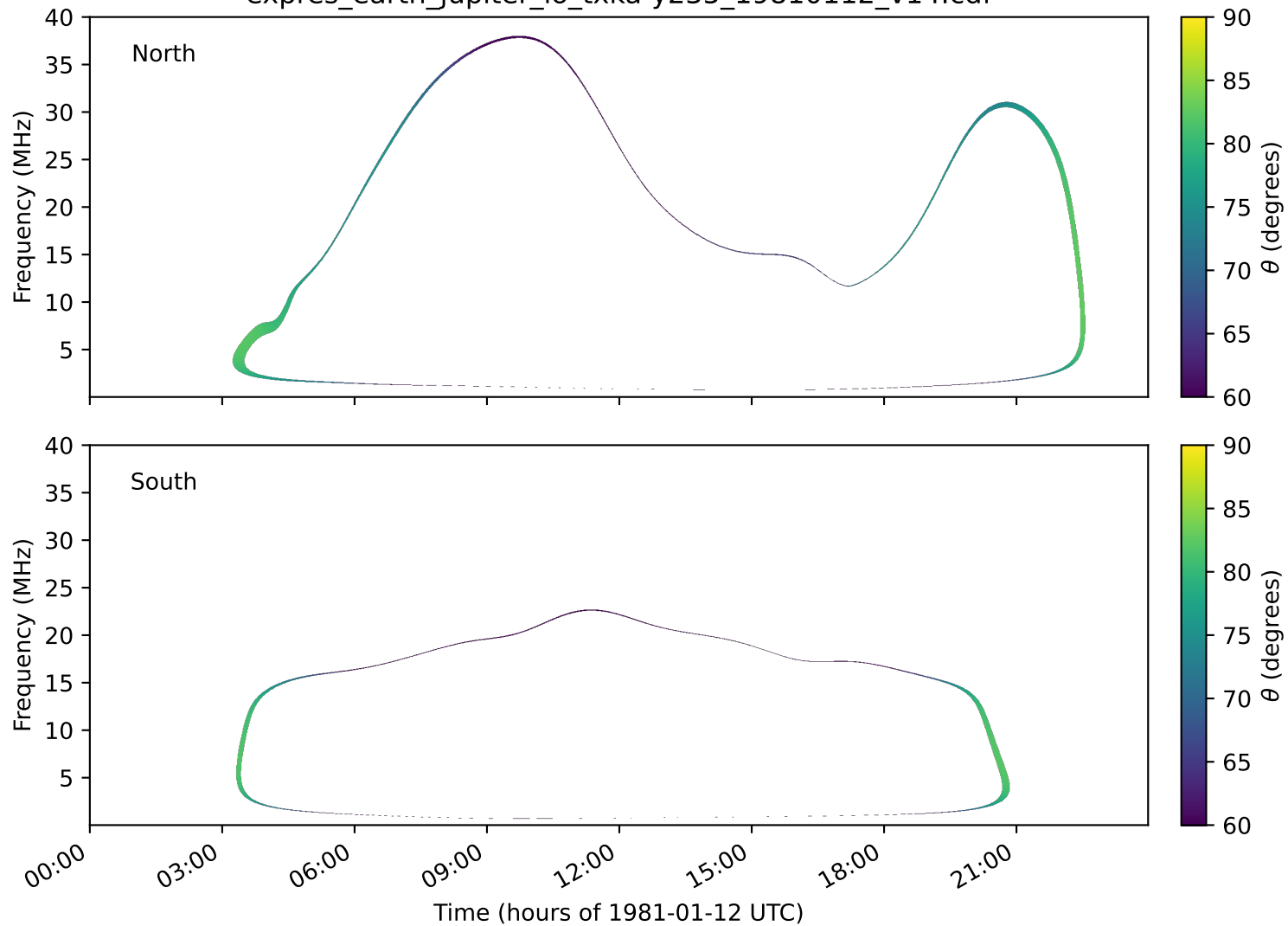
expres_earth_jupiter_io_txka-y235_19810112_v14.cdf
