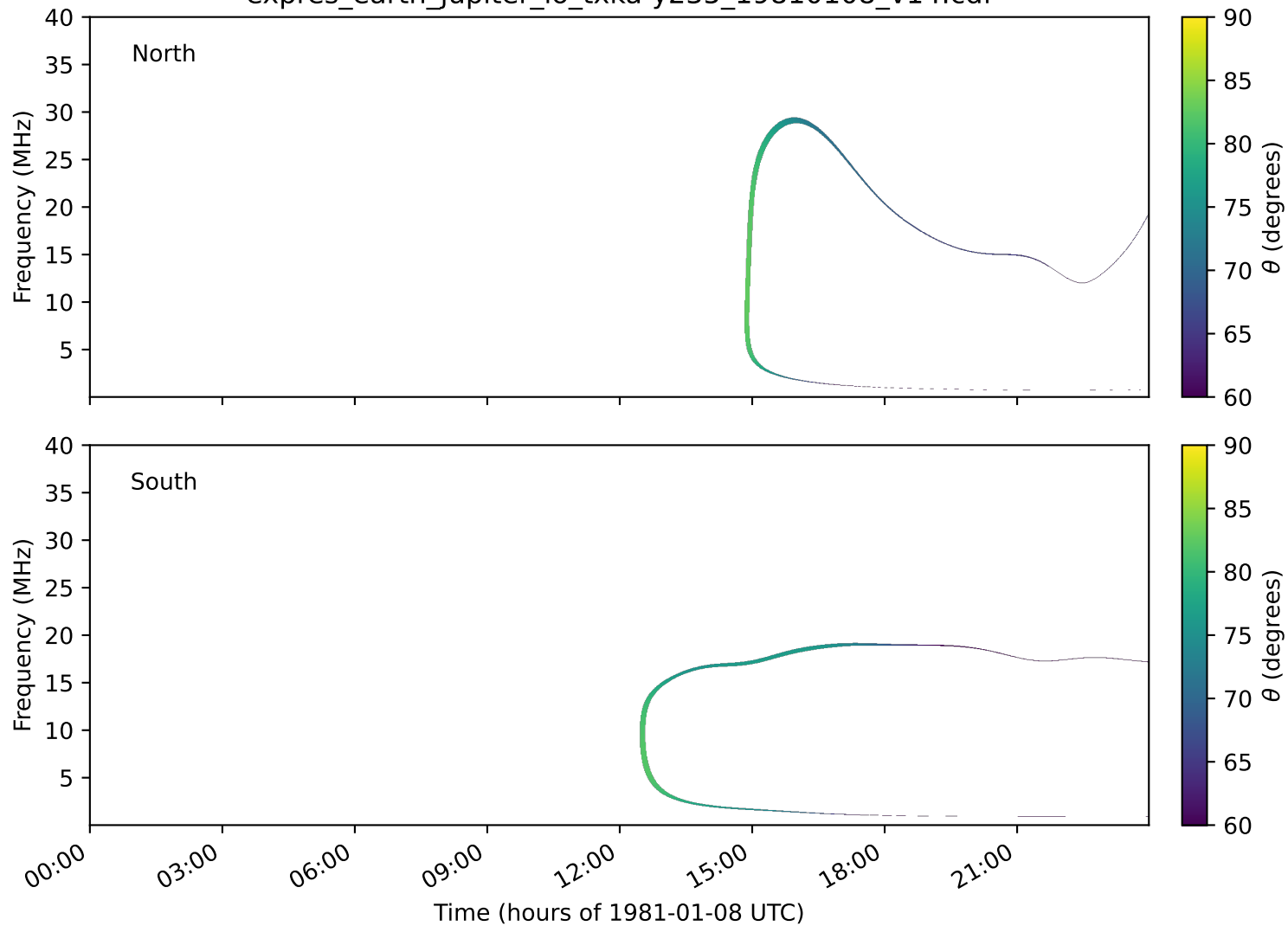
expres_earth_jupiter_io_txka-y235_19810108_v14.cdf
