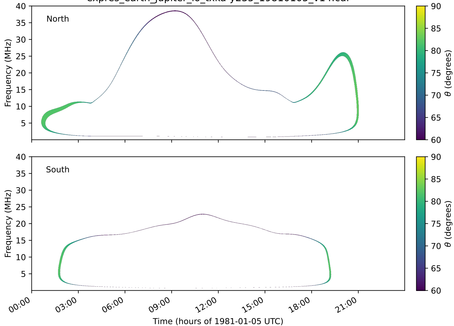
expres_earth_jupiter_io_txka-y235_19810105_v14.cdf
