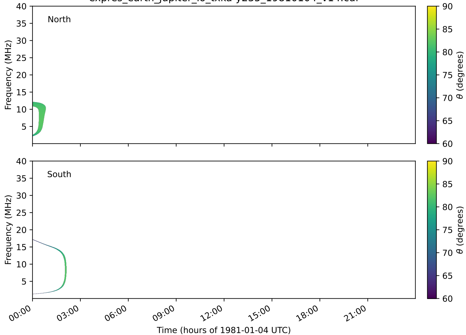
expres_earth_jupiter_io_txka-y235_19810104_v14.cdf
