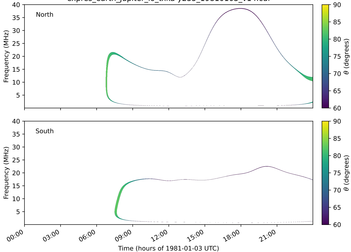
expres_earth_jupiter_io_txka-y235_19810103_v14.cdf
