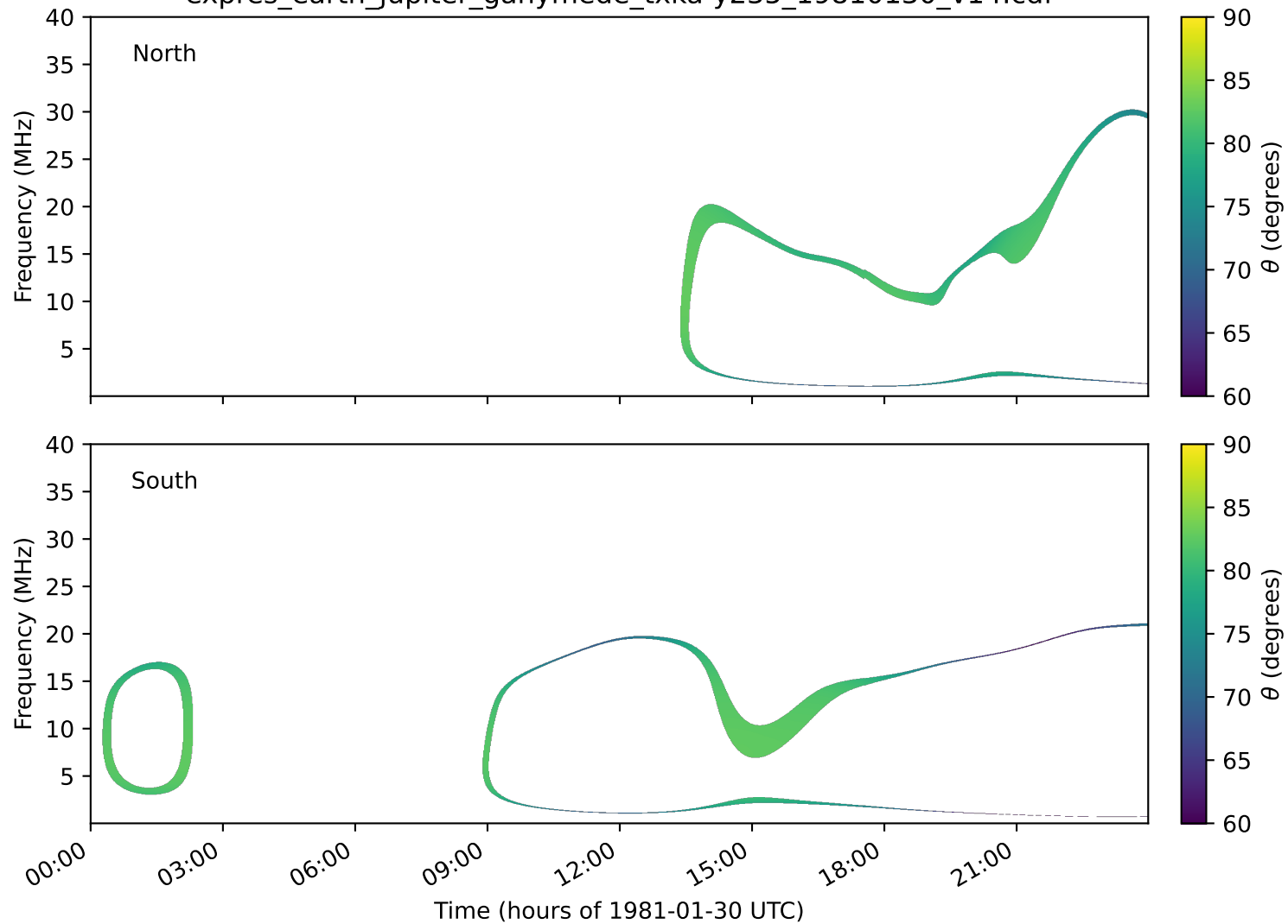
expres_earth_jupiter_ganymede_txka-y235_19810130_v14.cdf
