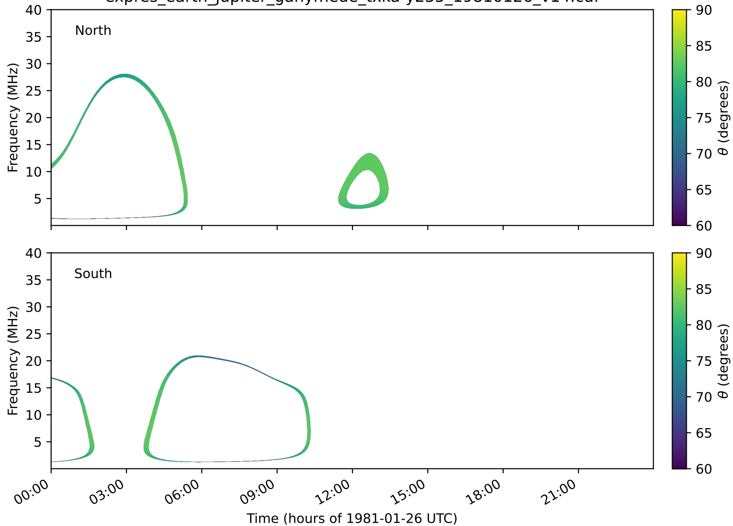
expres_earth_jupiter_ganymede_txka-y235_19810126_v14.cdf
