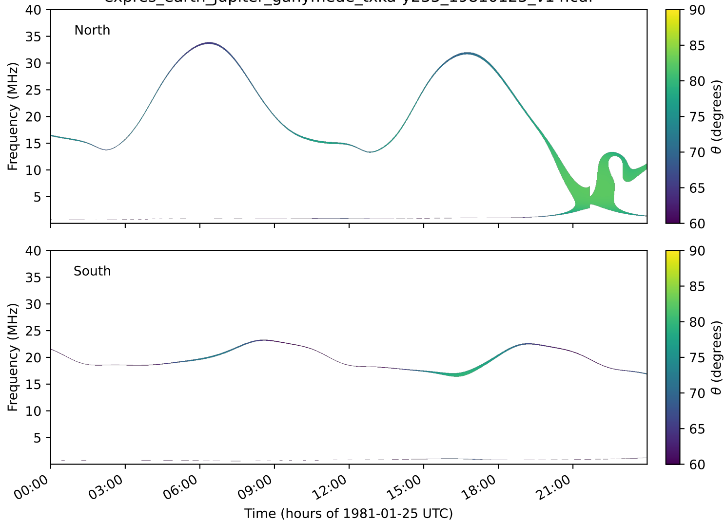
expres_earth_jupiter_ganymede_txka-y235_19810125_v14.cdf
