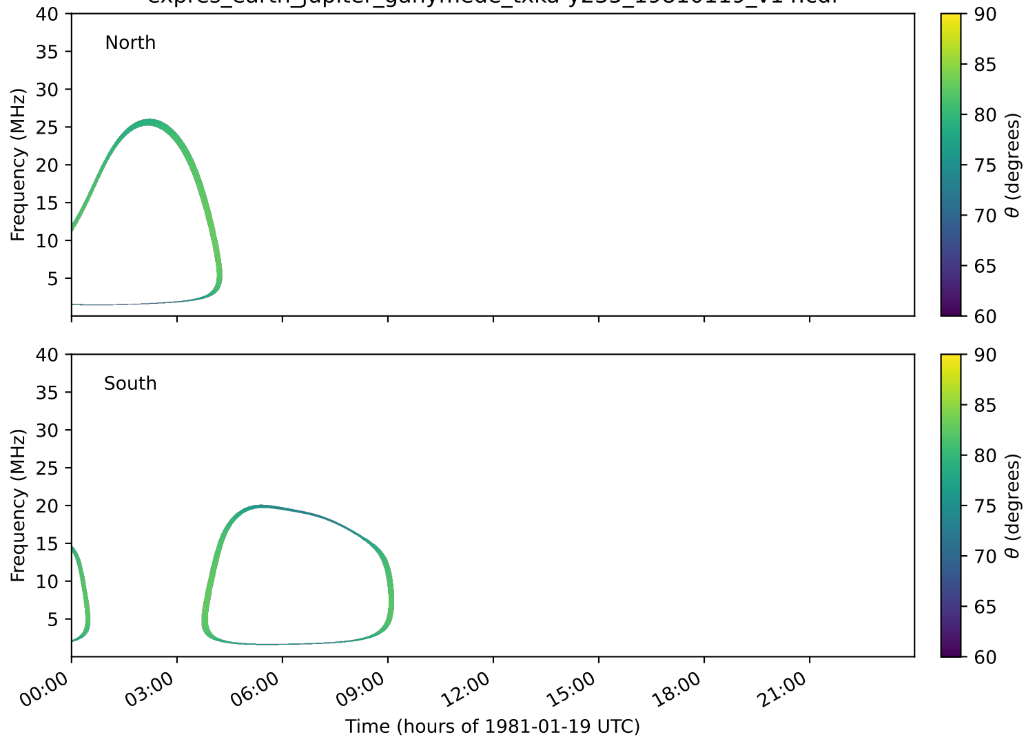
expres_earth_jupiter_ganymede_txka-y235_19810119_v14.cdf
