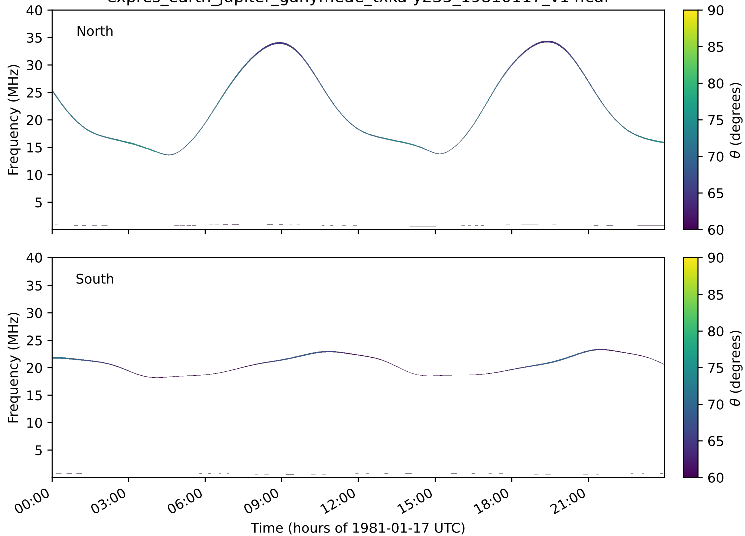
expres_earth_jupiter_ganymede_txka-y235_19810117_v14.cdf
