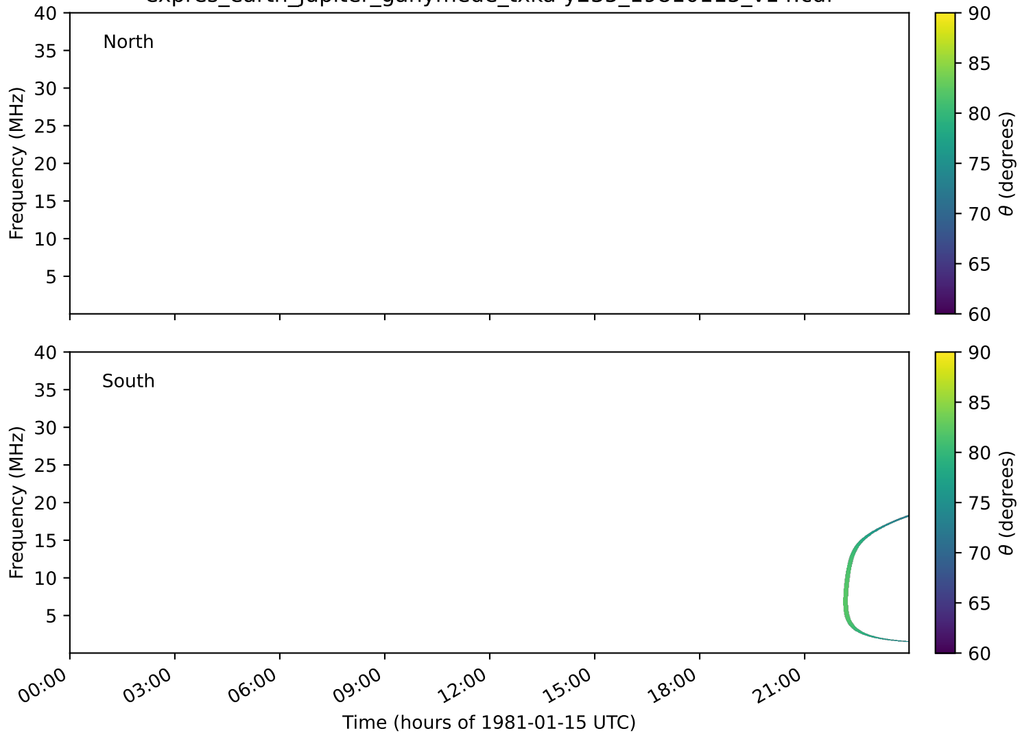
expres_earth_jupiter_ganymede_txka-y235_19810115_v14.cdf
