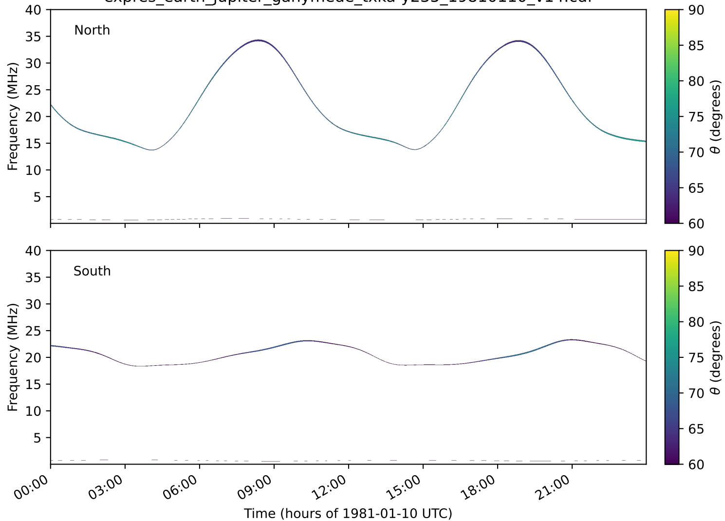
expres_earth_jupiter_ganymede_txka-y235_19810110_v14.cdf
