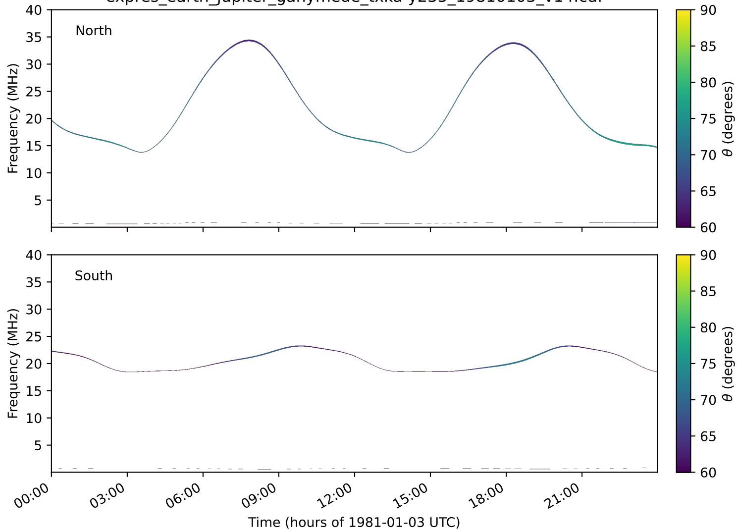
expres_earth_jupiter_ganymede_txka-y235_19810103_v14.cdf
