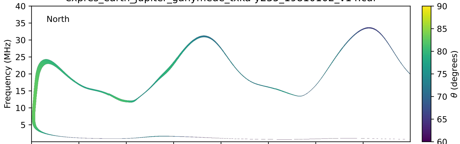
expres_earth_jupiter_ganymede_txka-y235_19810102_v14.cdf
