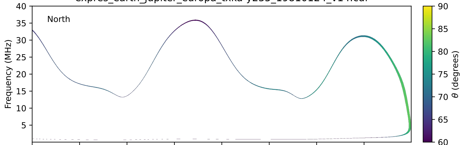
expres_earth_jupiter_europa_txka-y235_19810124_v14.cdf
