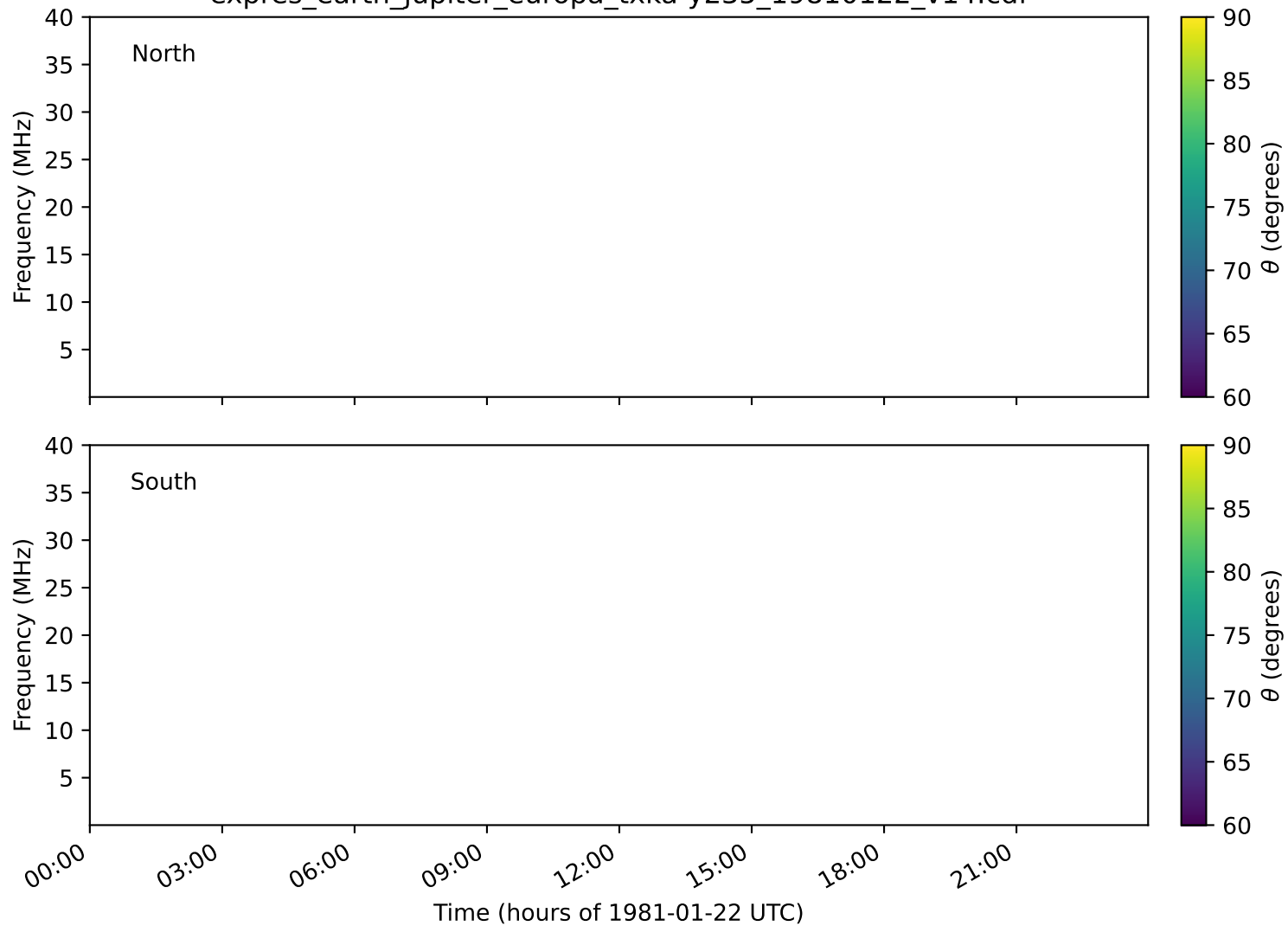
expres_earth_jupiter_europa_txka-y235_19810122_v14.cdf
