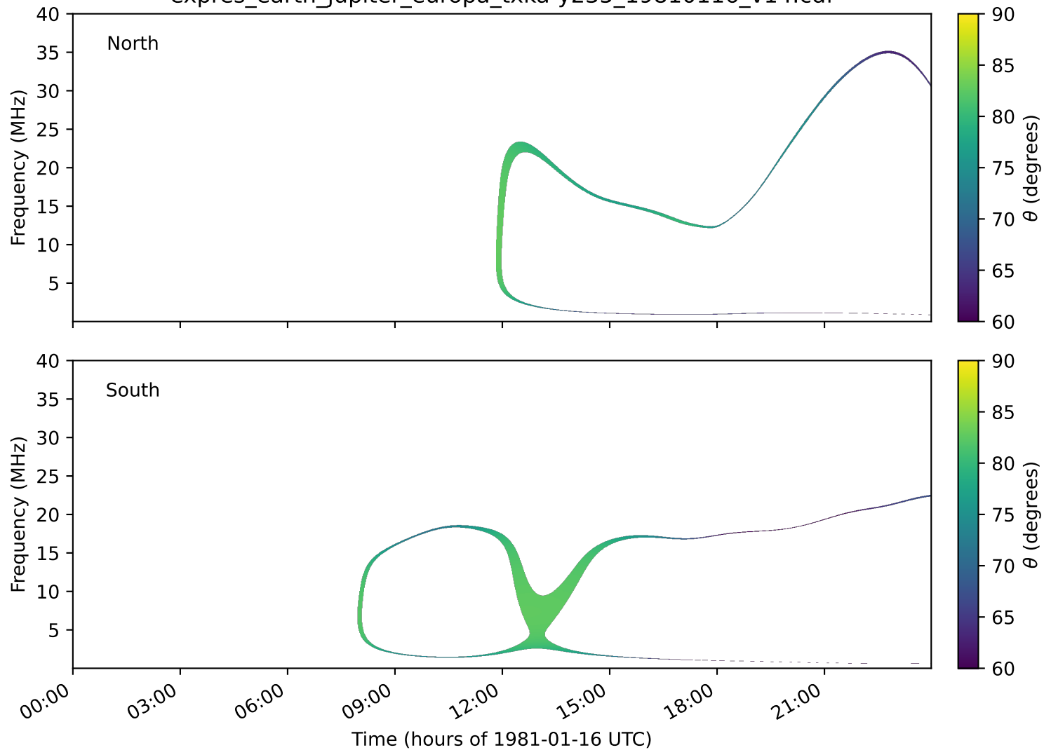
expres_earth_jupiter_europa_txka-y235_19810116_v14.cdf
