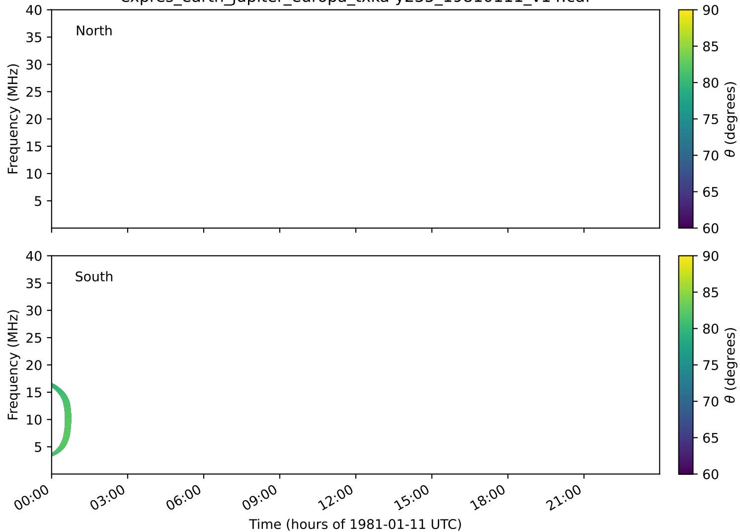
expres_earth_jupiter_europa_txka-y235_19810111_v14.cdf
