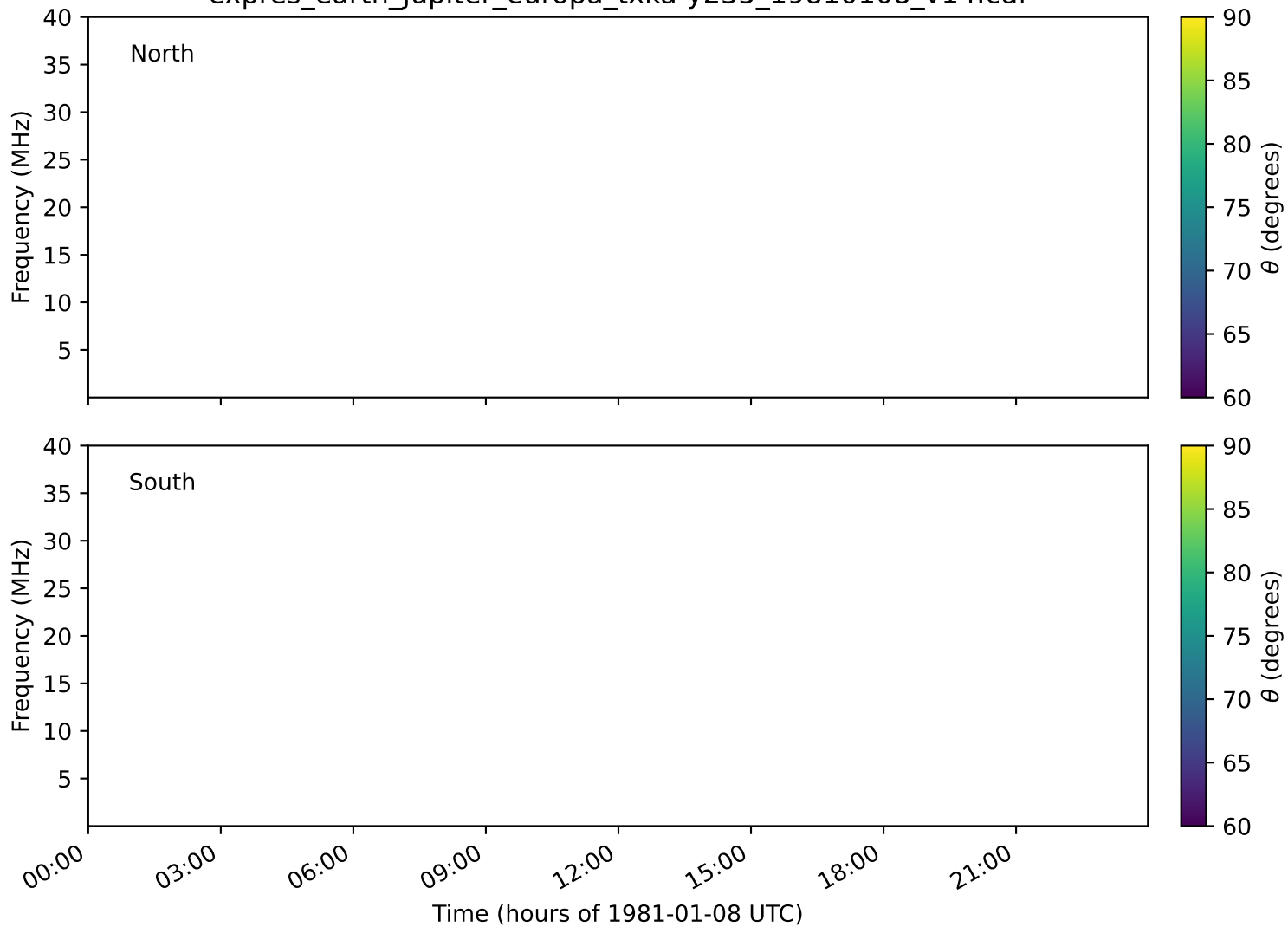
expres_earth_jupiter_europa_txka-y235_19810108_v14.cdf
