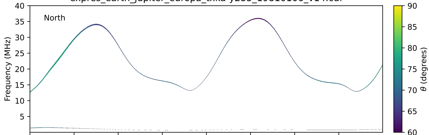
expres_earth_jupiter_europa_txka-y235_19810106_v14.cdf
