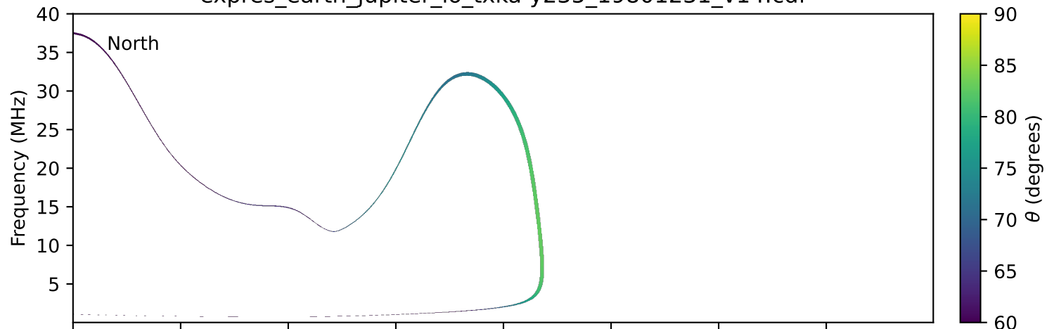
expres_earth_jupiter_io_txka-y235_19801231_v14.cdf
