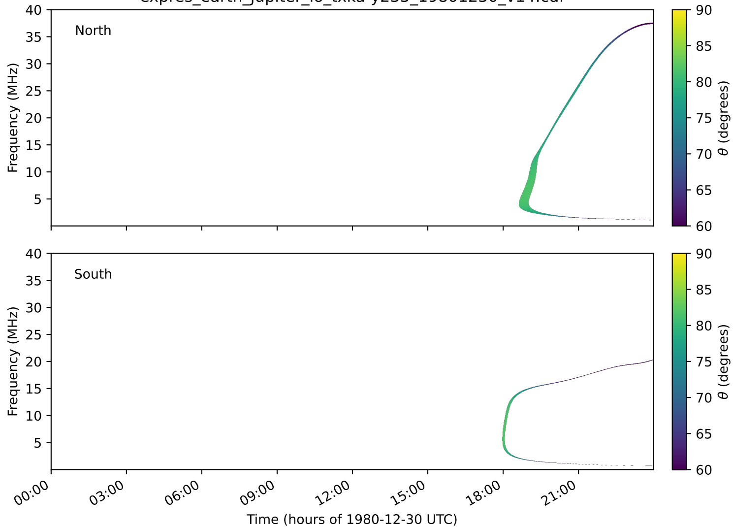
expres_earth_jupiter_io_txka-y235_19801230_v14.cdf
