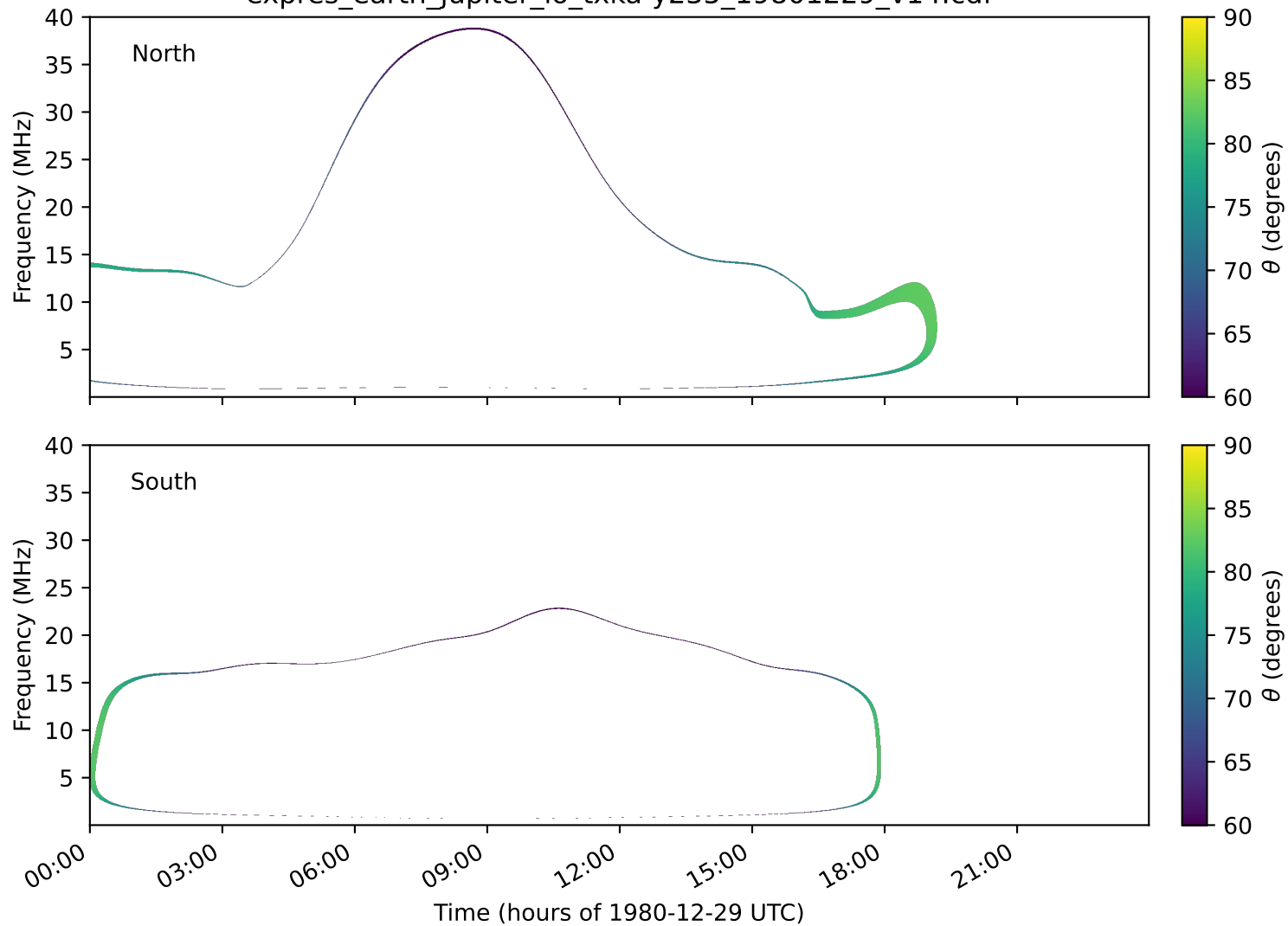
expres_earth_jupiter_io_txka-y235_19801229_v14.cdf
