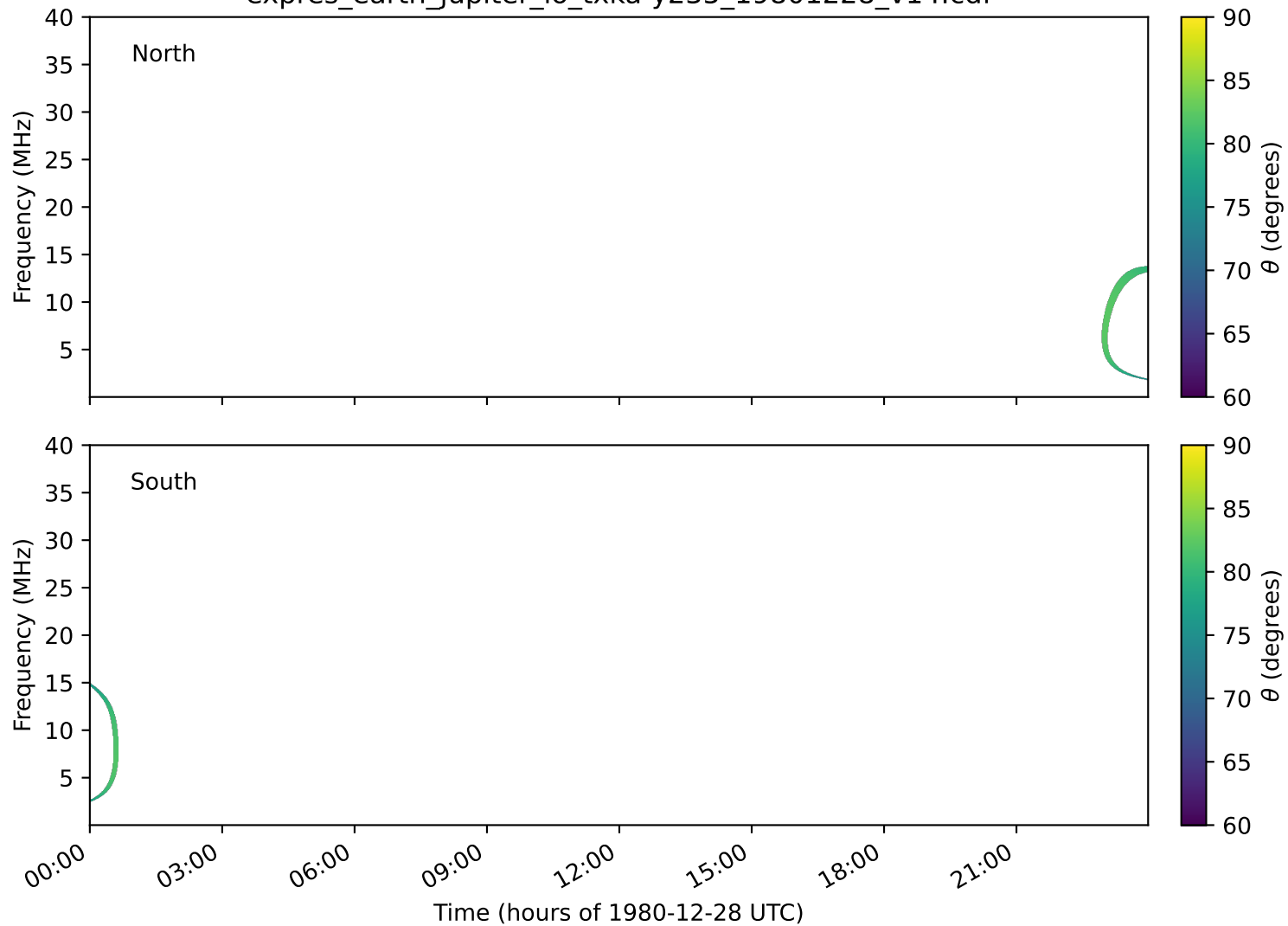
expres_earth_jupiter_io_txka-y235_19801228_v14.cdf
