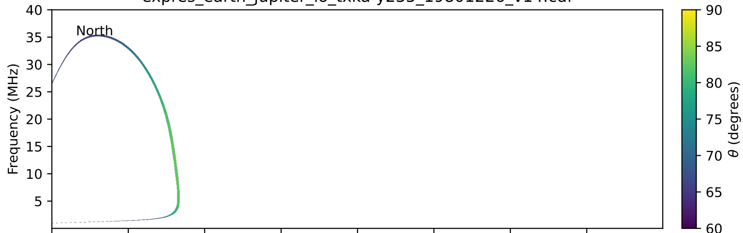
expres_earth_jupiter_io_txka-y235_19801226_v14.cdf
