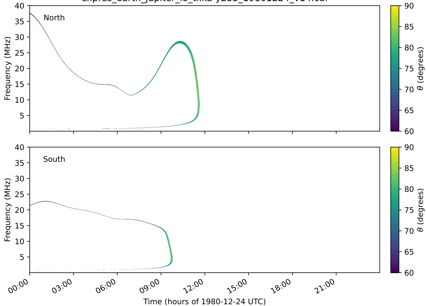
expres_earth_jupiter_io_txka-y235_19801224_v14.cdf
