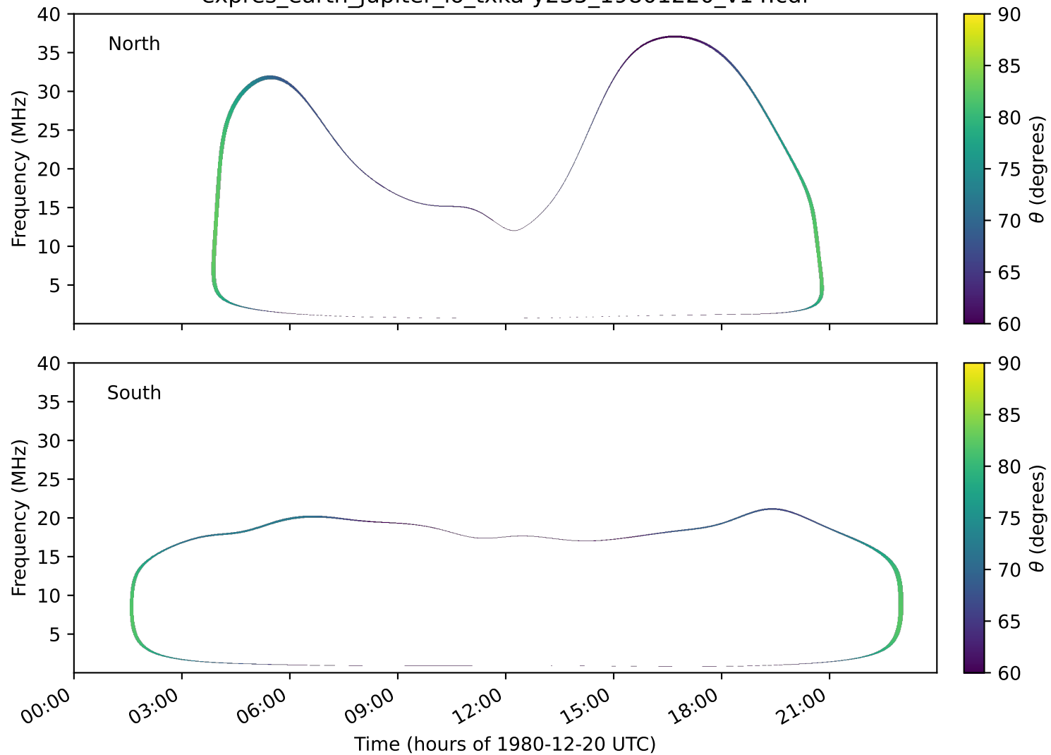
expres_earth_jupiter_io_txka-y235_19801220_v14.cdf
