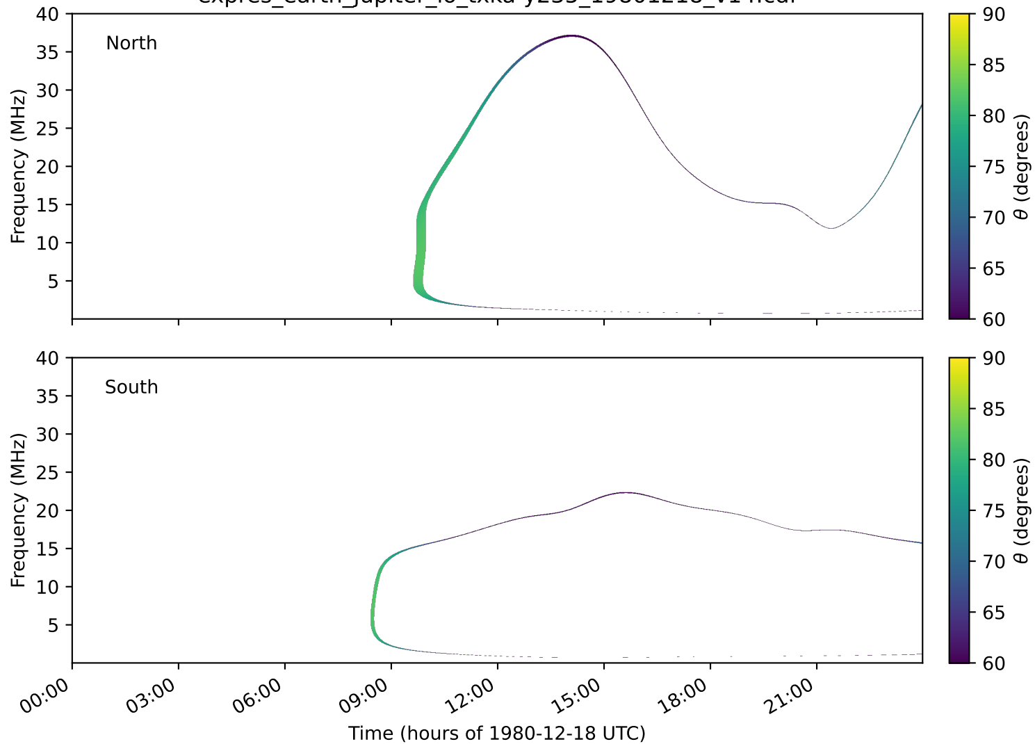
expres_earth_jupiter_io_txka-y235_19801218_v14.cdf
