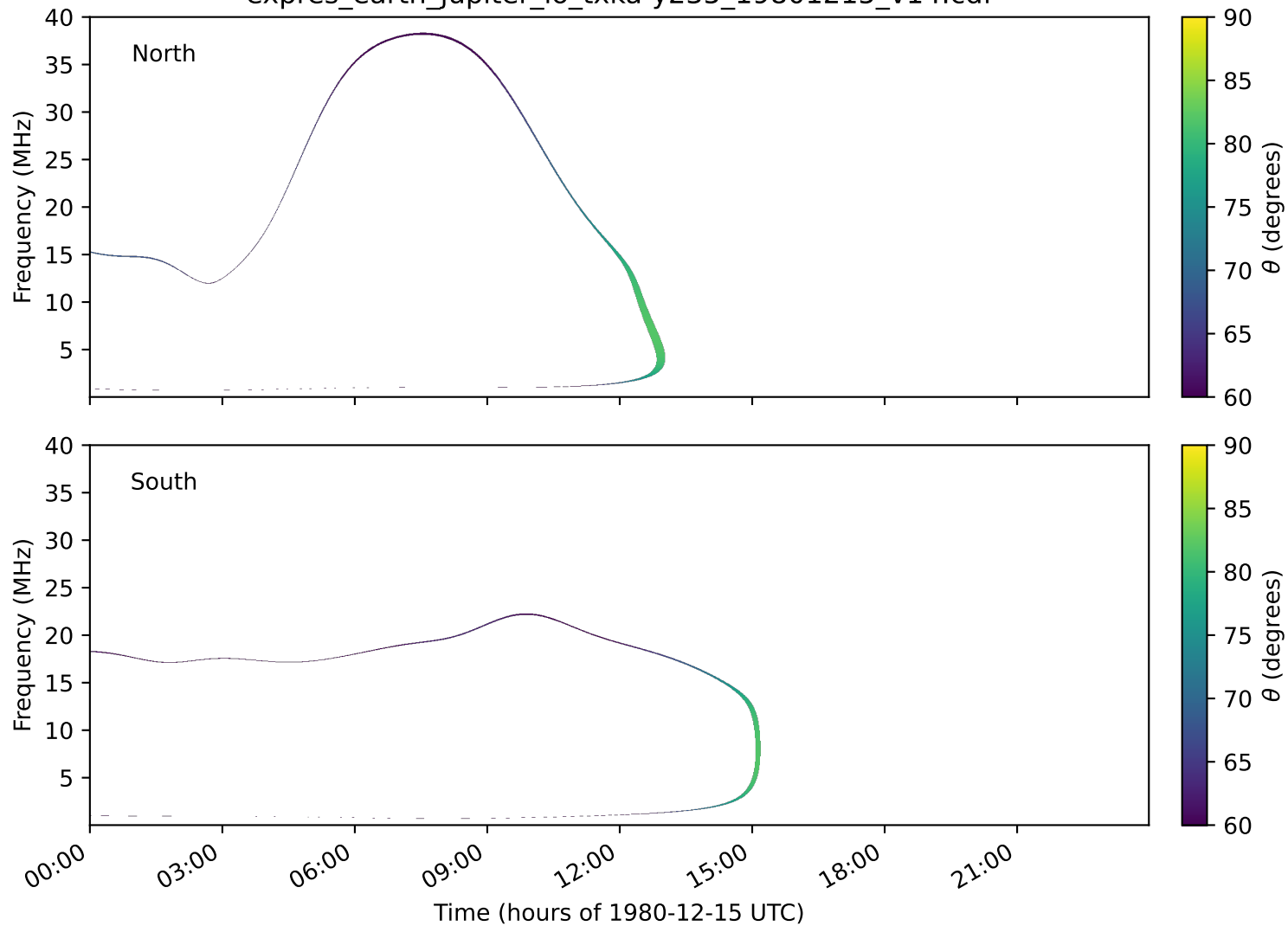
expres_earth_jupiter_io_txka-y235_19801215_v14.cdf
