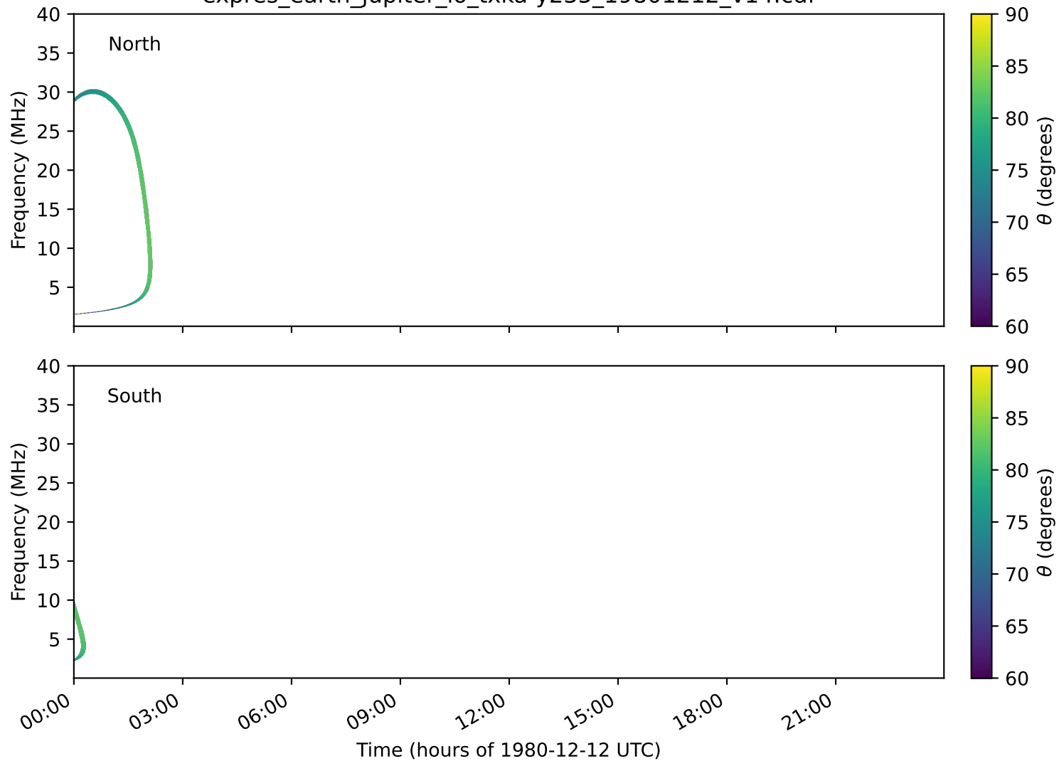
expres_earth_jupiter_io_txka-y235_19801212_v14.cdf
